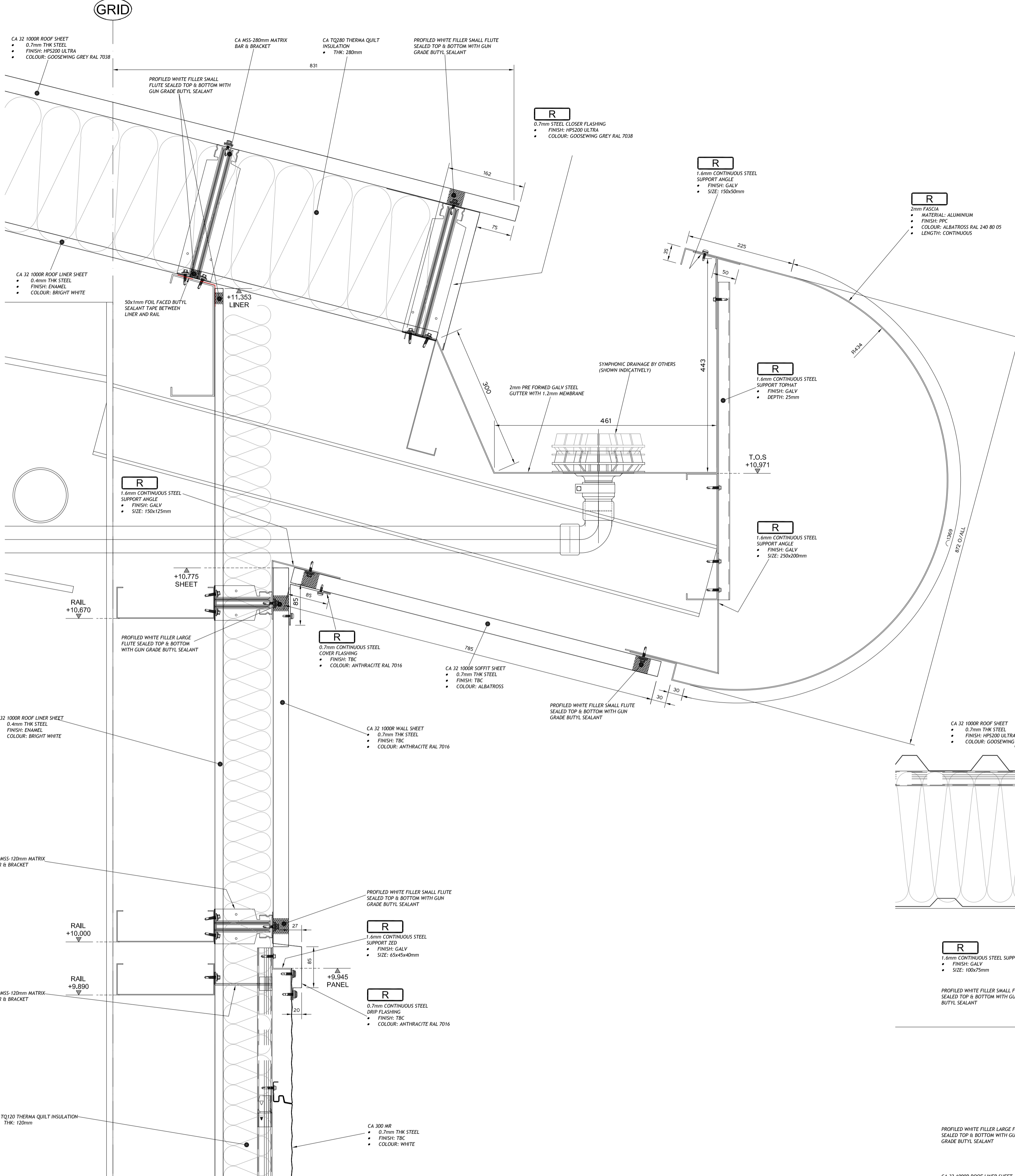
D01/1 - EAVES DETAIL 1:5
